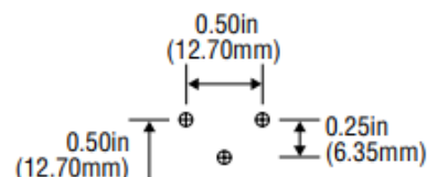
Cut-Out for 4578/4788/6747/6748
