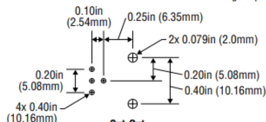
Cut-Out for 6717/6718
