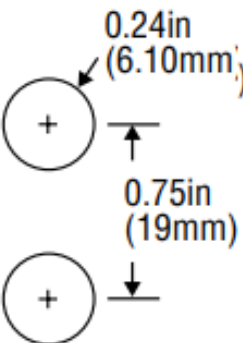
Panel Cut-Out for 6883/6884
