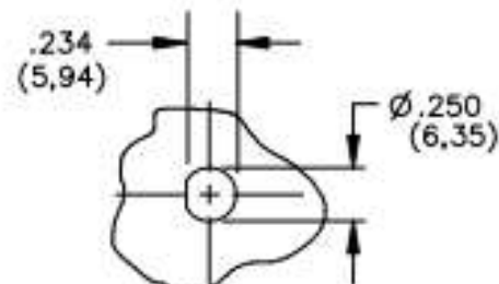
PANEL CUTOUT
