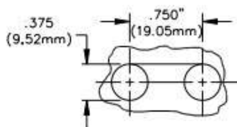
PANEL CUTOUT
